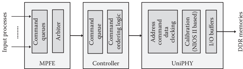
FIGURE 2.20 Arria 10 hard memory controller.
