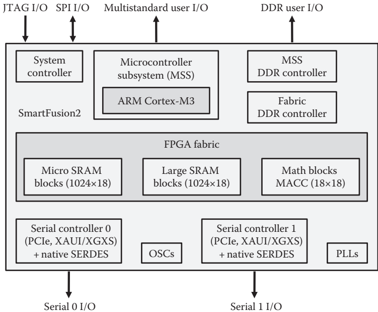
FIGURE 3.12 SmartFusion architecture.
